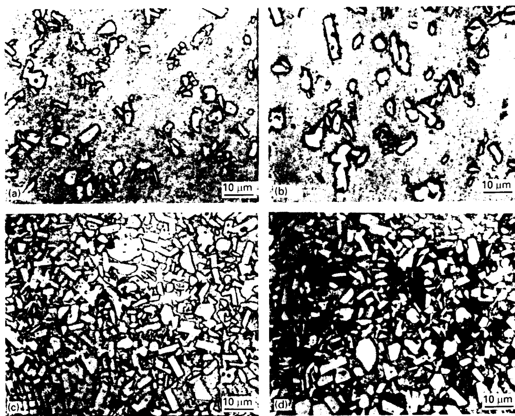
Figure 2 Optical micrographs of the Cu/TiB 2 platelet composites made by the two methods: (a) 15 vol % TiB 2 coated filler method; (b) 15 vol % TiB 2 admixture method; (c) 60 vol % TiB 2 coated filler method; (d) 60 vol % TiB 2 admixture method.
