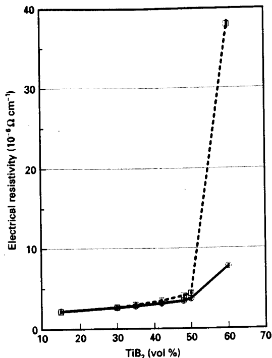
Figure 9 Variation of electrical resistivity with TiB 2 platelet volume fraction in copper-matrix composites made by (○) the coated filler method and (□) the admixture method. The vertical bar at each data point is an error bar.
