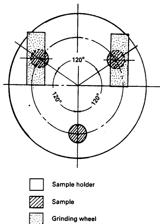
Figure 1 Abrasive wear testing geometry.
