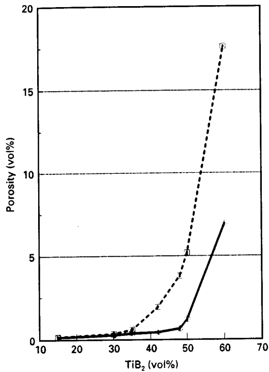
Figure 3 Variation of porosity with \text{TiB}_2 platelet volume fraction in copper-matrix composites made by (○) the coated filler method and (□) the admixture method. The vertical bar at each data point is an error bar.
