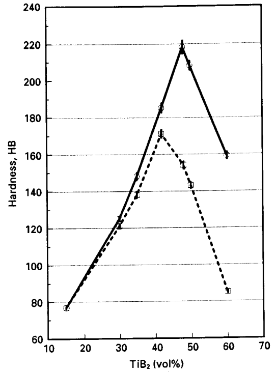
Figure 5 Variation of Brinell hardness with \text{TiB}_2 platelet volume fraction in copper-matrix composites made by (○) the coated filler method and (□) the admixture method. The vertical bar at each data point is an error bar.
