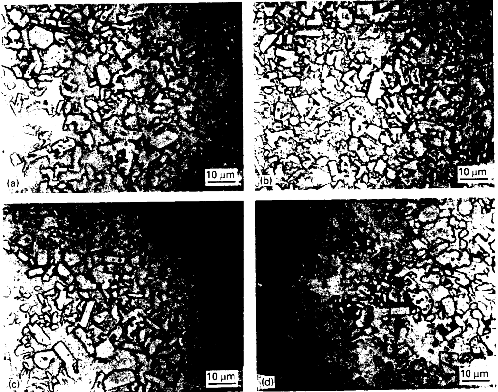
Figure 4 Optical micrographs of the Cu \text{TiB}_2 platelet composites made by the two methods: (a) 42 vol % \text{TiB}_2 coated filler method; (b) 42 vol % \text{TiB}_2 , admixture method; (c) 50 vol % \text{TiB}_2 , coated filler method; (d) 50 vol % \text{TiB}_2 , admixture method
